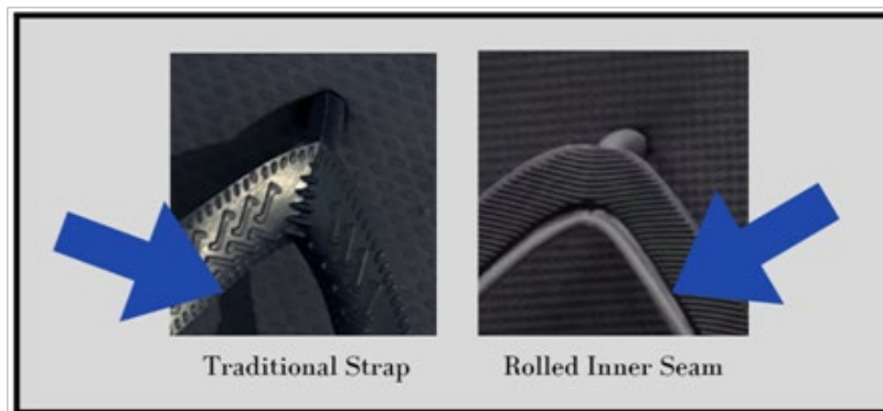
Picture 1: Comparison of Traditional Straight Edge Strap and Rolled Inner Seam Strap
