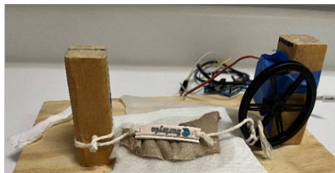
Picture 2: Apparatus to Simulate Strap Motion
