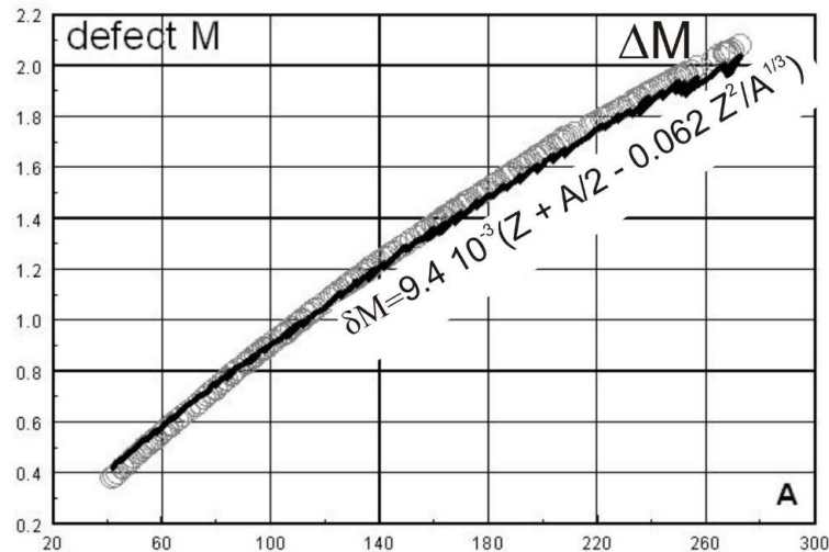
Figure 12: Comparison of calculated mass defects of nuclei (Eq.(111)) with experimentally measured values of \Delta M
