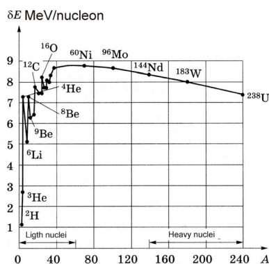
Figure 1: The Binding Energy per One Nucleon of the Nucleus
