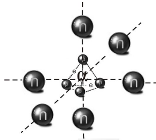
Figure 11: “Elementary cell” three-dimensional “crystal” models of a heavy nucleus in which alpha particles are “glued” together by neutrons.
