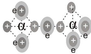
Figure 8: Schematic representation of energy bonds in the Be-9 core. Dotted lines represent the possibility of a relativistic electron jumping between protons.
