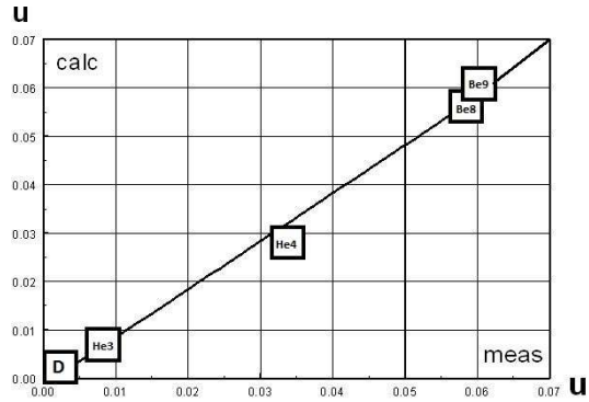
Figure 9: Comparison of calculated values of the mass defect of light nuclei with the measurement data
