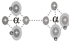
Figure 7: The schematic representation of energy bonds in the Be-8 core. Dotted lines represent the possibility of a relativistic electron jumping between protons.
