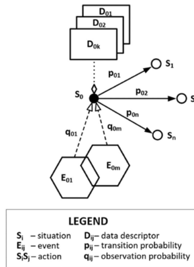
Figure 3: Inventory for Formulating Non-deterministic Rules
