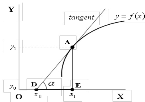
Figure 3: Material system “Segment of line y = f(x) right-angled triangle \triangle DAE ” in the Cartesian coordinate system XOY . The tangent \overline{DA} is the hypotenuse of the right-angled triangle \triangle DAE . The constants x_0, x_1, y_0, y_1 are the abscissas and ordinates of the points D, A, E . The quantities \Delta x_{1,0} \equiv x_1 - x_0 \neq 0 and determine the lengths of the legs of the triangle \triangle DAE .
