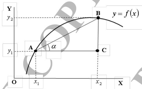
Figure 2: Material system “Segment of the line y = f(x) + right-angled triangle \triangle ABC ” in the Cartesian coordinate system XOY . The secant \overline{AB} is the hypotenuse of the right-angled triangle \triangle ABC . Quantities x_1, x_2, y_1, y_2 are the abscissas and ordinates of the points A, B, C , respectively.
