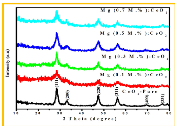
Figure 1: X-ray diffraction patterns of pure and Mg 2+ (0.1, 0.3, 0.5
