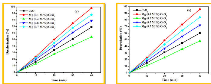
Figures 3: percentage (a) degradation and (b) decolorization of pure and Mg^{2+} (0.1, 0.3, 0.5 and 0.7 M.%) doped CeO_2 quantum dots.
