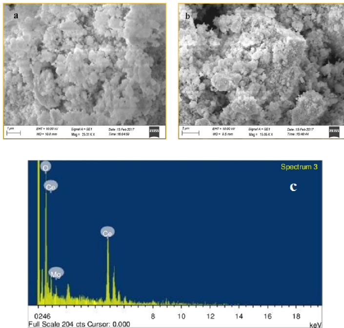
Figure 2: SEM image of (a) pure CeO_2 and (b) doped with Mg^{2+} (0.1 M.%) quantum dots (c) EDX
