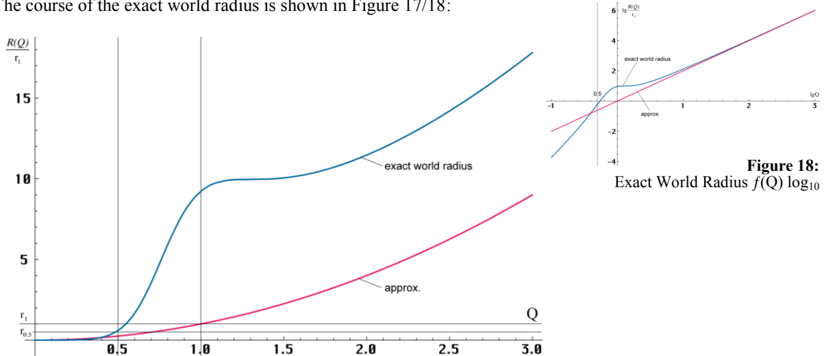
Figure 17: Exact World Radius f(Q) Linear
