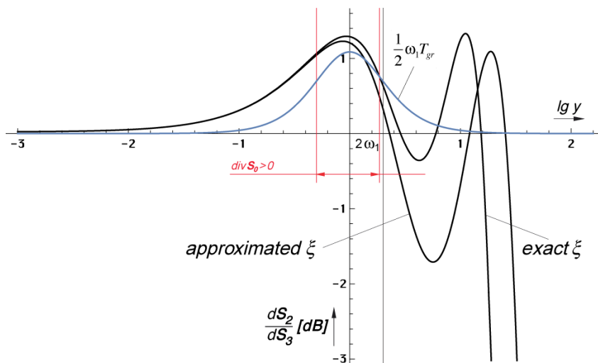
Figure 9: Relative Offset Between Approximation and Radiation Law in Dependence of the Function \xi Used
