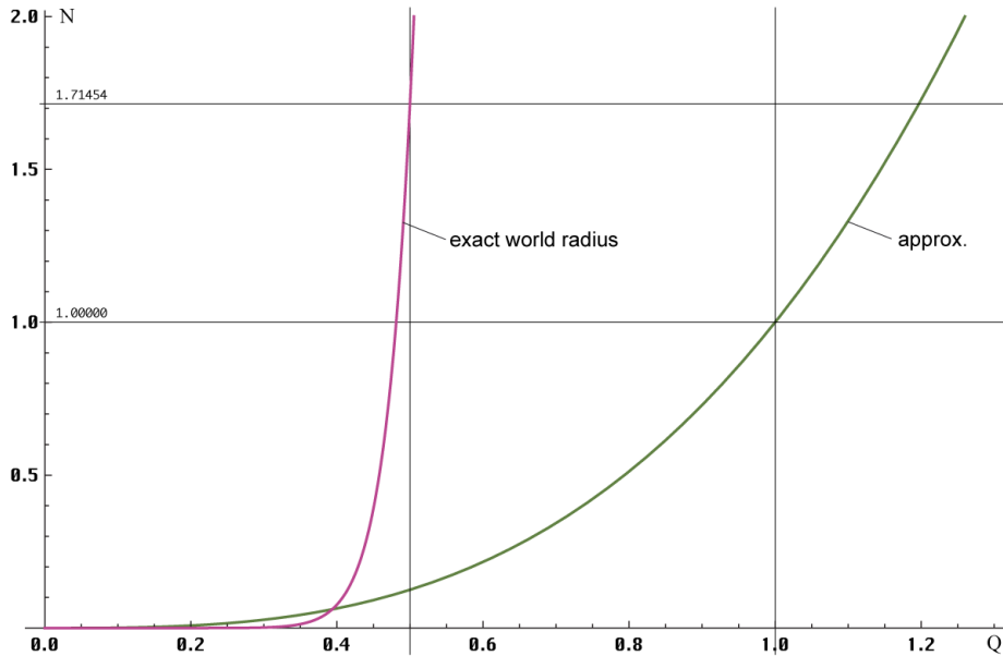
Figure 19: Maximum Possible Number of Line Elements N in the Universe at the Beginning of Expansion
