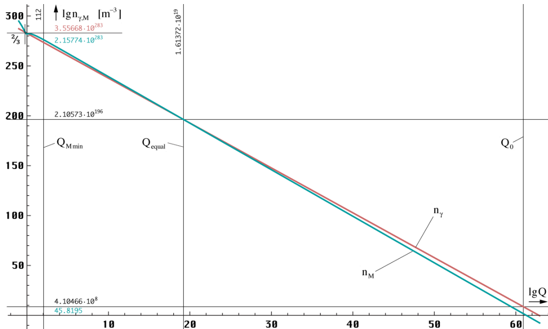
Figure 23: Photon-Number-Density in Comparison to the Nucleon-Number-Density of the CMBR per m^3
