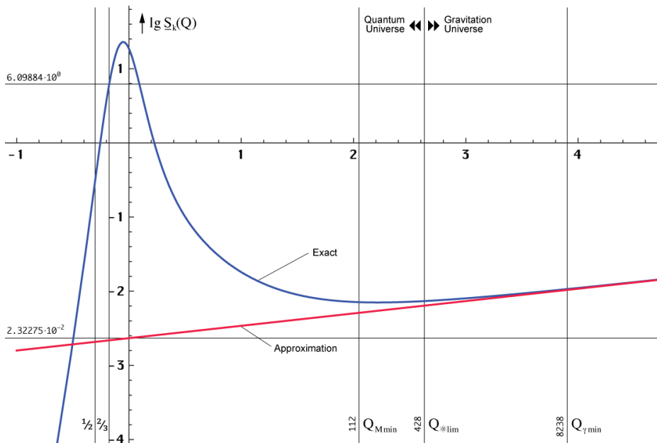
Figure 22: Entropy per Nucleon of the CMBR Small Scale
