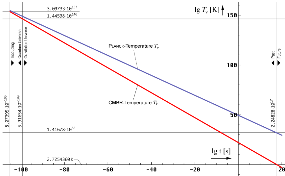
Figure 16a: Temporal Course of the CMBR Radiation-Temperature in Comparison With the PLANCK-Temperature from Incoupling until Now
