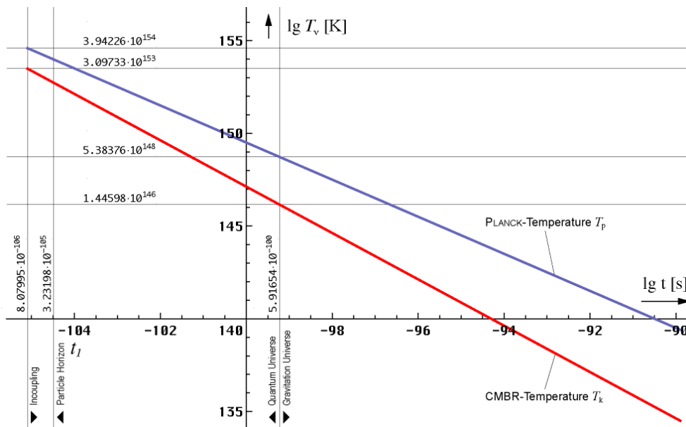
Figure 16b: Temporal Course of the Radiation-Temperature of the CMBR in Comparison With the PLANCK-Temperature Shortly after BB
