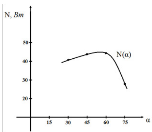
Figure 3: Power Dependence on Blade Installation Angle
