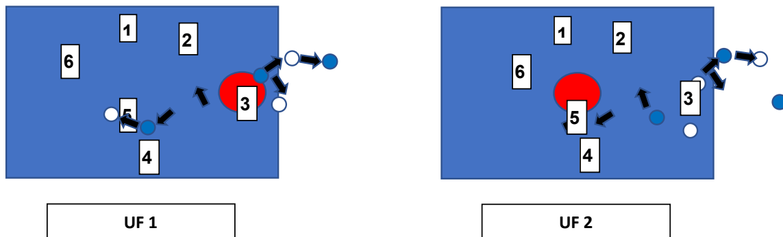
Figure 1: "G-D's Physics" Alternative Explanation for "Curved Space-Time".
